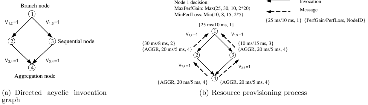
Figure 5: Resource provisioning in directed acyclic graphs
