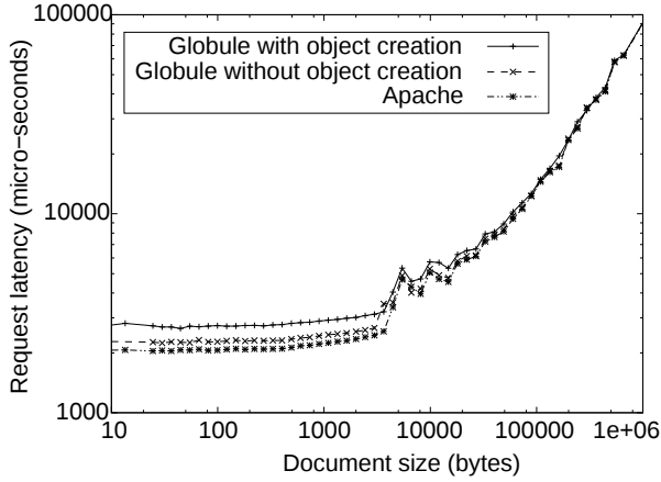
Figure 3. Request latencies
